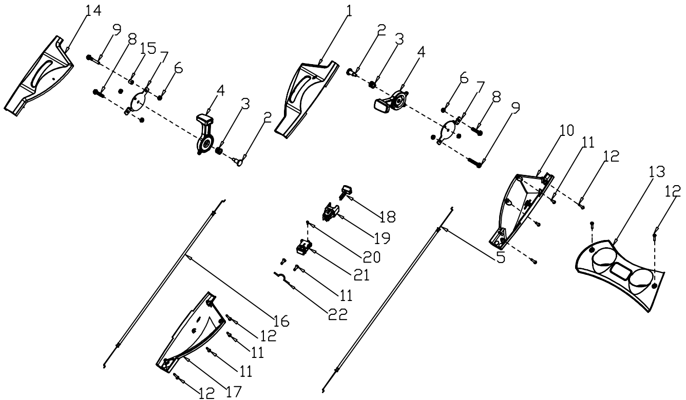
Drawing C
